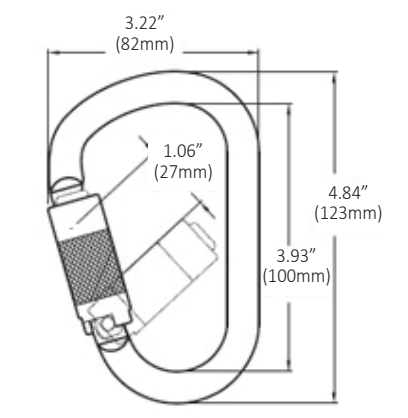
#354-4 Steel twist-lock carabiner, 1" gate Proof loaded to 3,600 lbs. Minimum. breaking load: 5,000 lbs.
