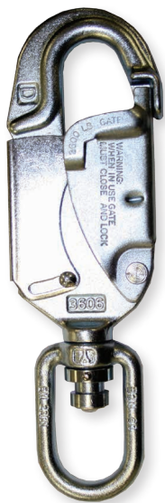
#RL-28 Steel swivel locking snaphook, 3/4" gate Impact Indicator Proof loaded to 3,600 lbs.
