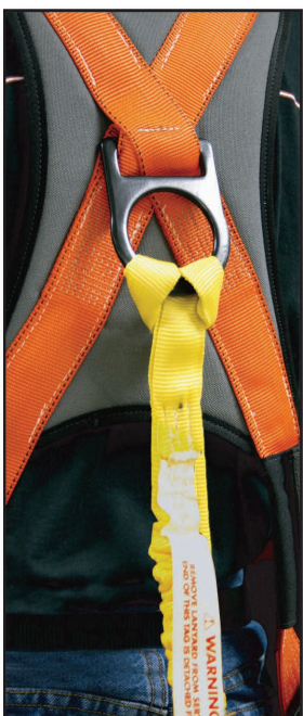
Choke-Loop 2 Internal shock absorber Looped end
