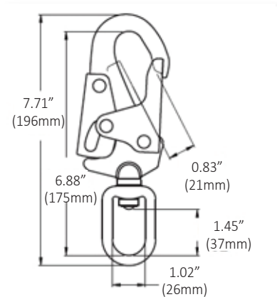
#49 Steel swivel locking snaphook, 3/4" gate Proof loaded to 3,600 lbs. Minimum. breaking load: 5,000 lbs.
