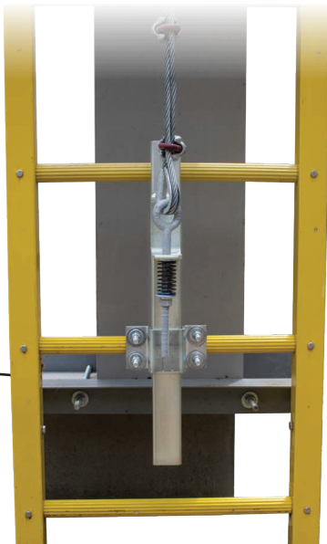
Bottom Bracket & Tensioner
