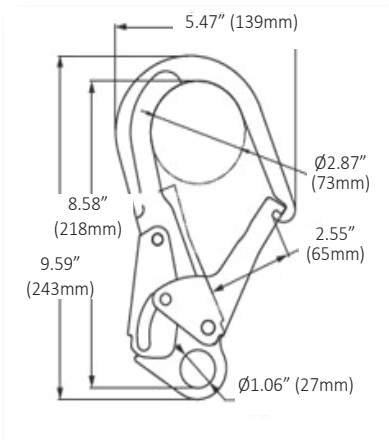
#Z136 Steel locking rebar snaphook, 2 1/2" gate Proof loaded up to 3,600 lbs. Minimum breaking load: 5,000 lbs.
