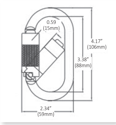
354-6TL Steel twist-lock carabiner, 3/4" gate Proof loaded up to 3,600 lbs. Min. breaking load: 5,000 lbs.
