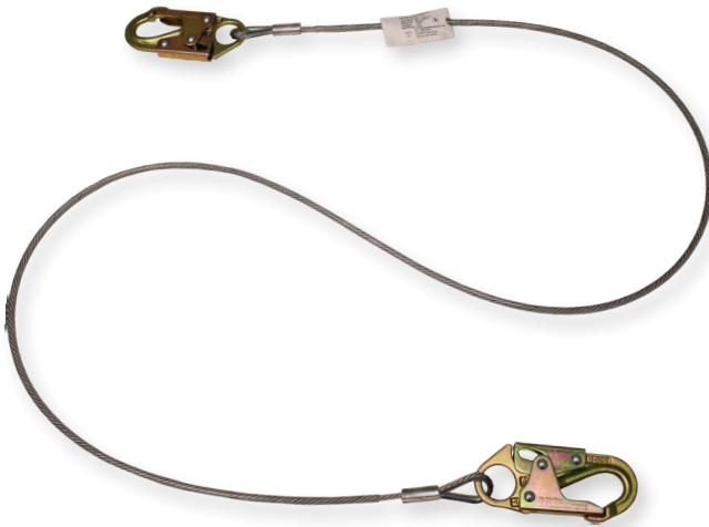
470 7/32" vinyl coated 6' wire rope lanyard #Z74 locking snaphooks at each end
