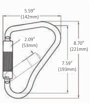
#62 Steel twist-lock scaffold hook, 2" gate Proof loaded to 3,600 lbs. Minimum breaking load: 5,000 lbs.
