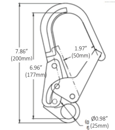
#69 Steel locking rebar snaphook, 1 3/4" gate Proof loaded up to 3,600 lbs. Min. breaking load: 5,000 lbs.
