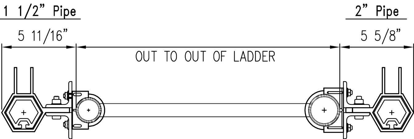
Welded Pipe Ladder
