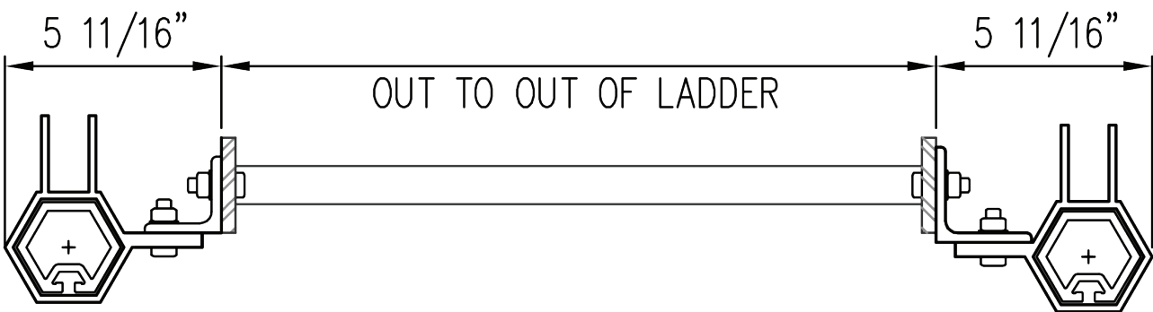
Flat Bar Ladder
