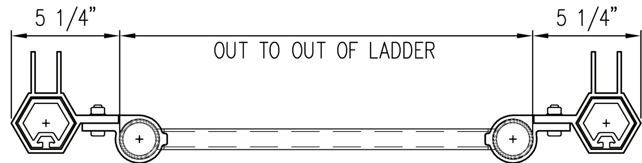
1-1/2" Pipe Ladder
