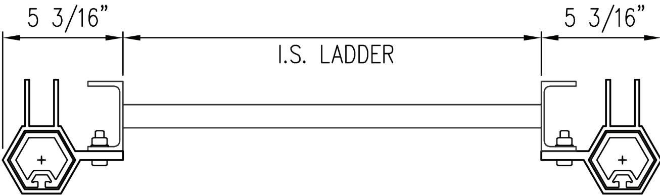
Channel Side Bar Ladder (Toeing Out)
