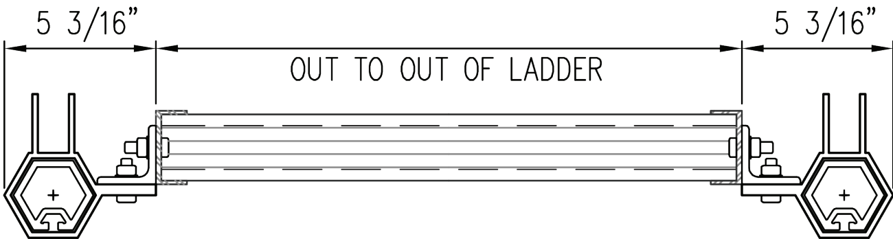
Channel Side Bar Ladder (Toeing In)
